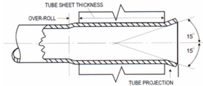
Over Roll & Flared Expansion
