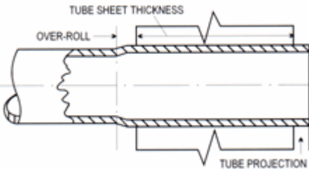
Over Roll Expansion
